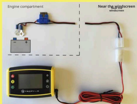
Automotive fuse holder / Automotive fuse holder
